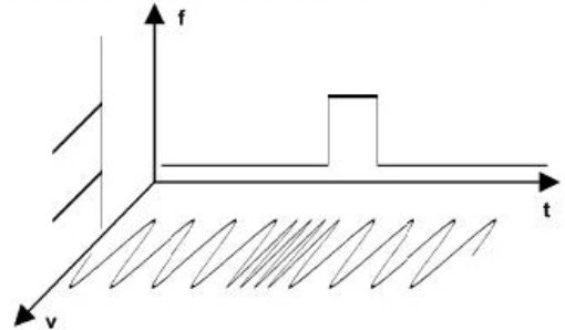
Figure 1. A sinewave signal with squarewave FM as shown on an oscilloscope (v vs. t), a spectrum analyzer (v vs. f) and a Modulation Domain Analyzer (f vs. t). These three instruments give a three dimensional view of the signal's properties.
