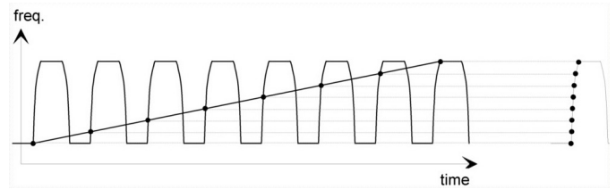
Figure 3. With repetitive sampling, many measurements are made at fairly long intervals and put together to show a fast frequency transition. Each measurement can be delayed down to 10 nsec with respect to the previous measurement.
