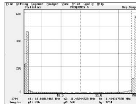
Figure 11. Jitter caused by a square wave frequency modulation gives a 2 bar distribution.
