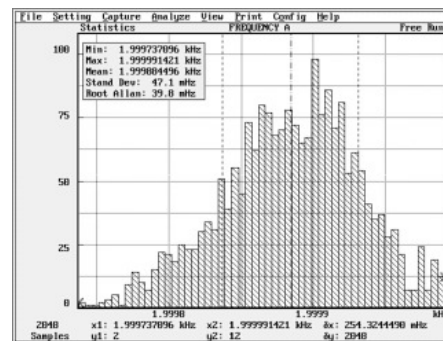
Figure 16. The histogram of frequency vs. time data indicates random noise.
