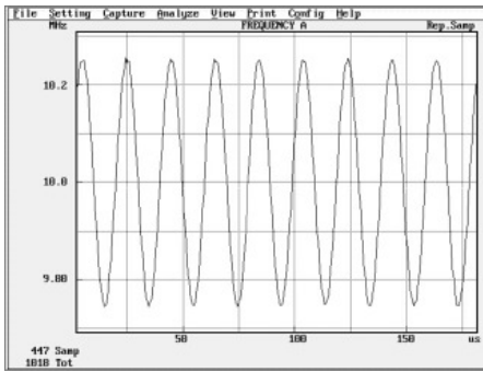
Figure 12. FM shown in the modulation domain. The modulation signal shape is revealed.
