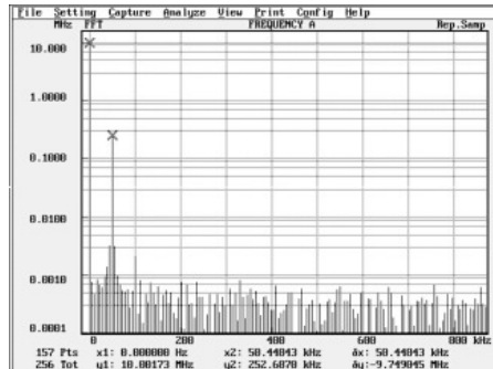
Figure 13. FFT processing of the modulation domain graph shows carrier, modulation frequency and deviation.
