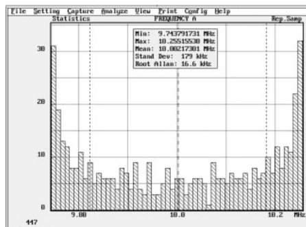
Figure 14. The distribution histogram shows frequency deviation and indicates sinusoidal modulation.
