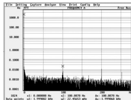
Figure 17. FFT-processing of the modulation domain graph shows the power supply contributed noise with a 100 Hz modulation.
